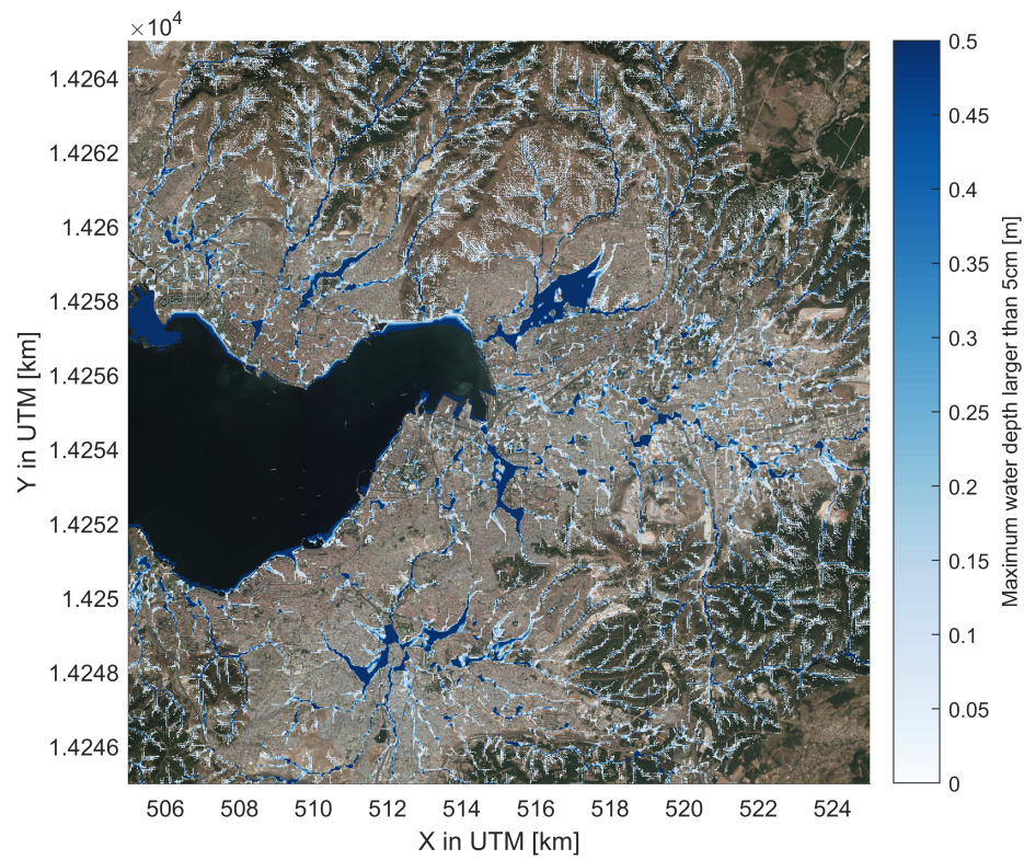
Fig. 1.7: SFINCS model for Izmir, Turkey
