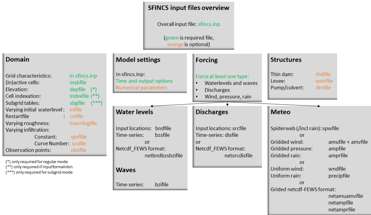
Fig. 1.12: Overview of input file of SFINCS with indication whther they are required or not
