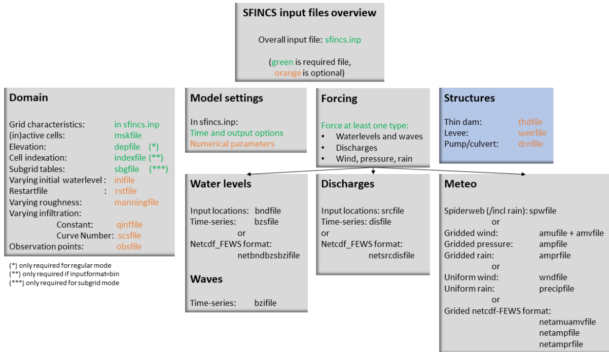
Fig. 1.18: Overview of input file of SFINCS with indication whether they are required or not
